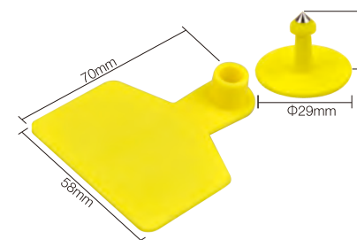
LD-7058A 8.2g/set
