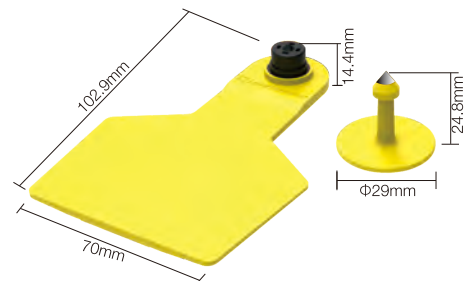
LD-2770A 10g/set
