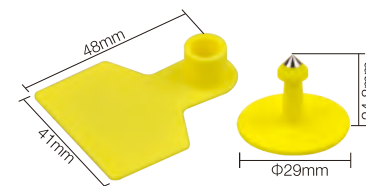
LD-4841A 4.7g/set
