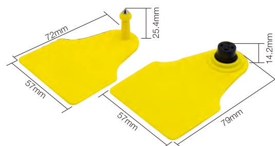
LD-7965AB 12.6g/set
