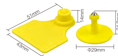
LD-5143A 6.1g/set
